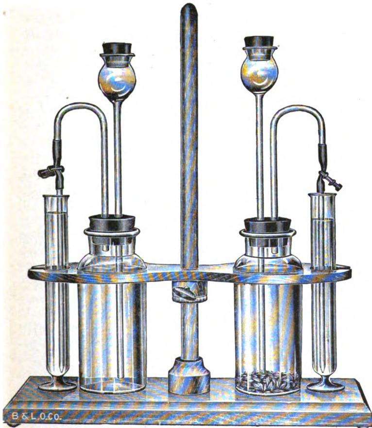
FIG. 115. — A respiroscope; \times \frac{1}{4} . While the seeds are germinating, the chamber is kept closed by the smaller rubber stopper and clamp, though these are removed in applying the test.
